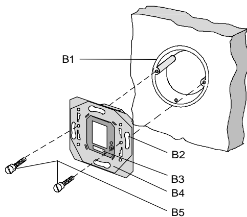
Figure 2: Mounting the shutter switch UP 520/01
