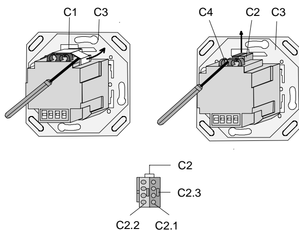
Figure 3: slipping off/on bus block
