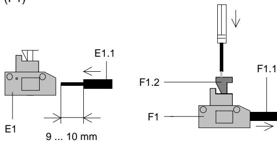
Figure 5: Connecting/disconnecting cables
